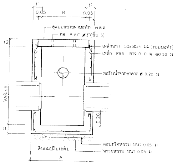
SECTION 1-1
